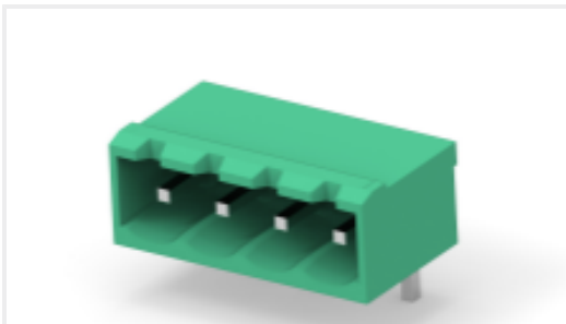
TE 产品编号2350513-4 4POS TB HDR 90 DEG, PITCH 5.0 & TL 4.5mm
