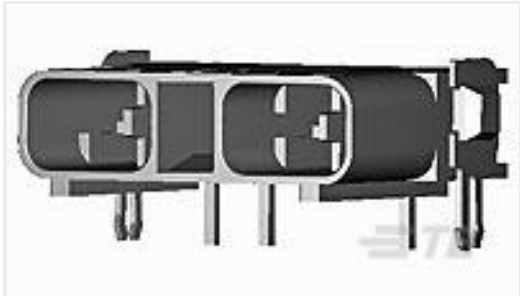
TE 产品编号2106111-6 Assembly, Right Angle TH Header, 4-Posit
