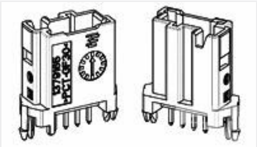
TE 产品编号1379165-4 4pos MQS .63 header 180deg THR
