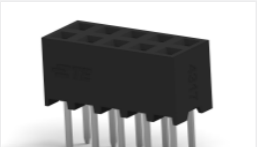
TE 产品编号1-2314824-0 10P,2MM,B-B,REC,DRV,T,2.7,0.1AU,TB,W/CAP
