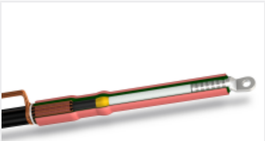
TE 产品编号000877-011 IXSU-F5151
