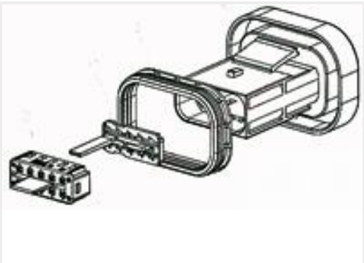
TE 产品编号1801610-2 BULK HEAD, MCON, 10W, CLIPPED
