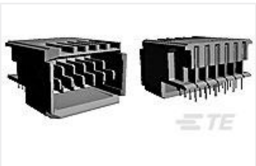
TE 产品编号5223964-6 UNV,PWR,MDL,HDR,SEQ
