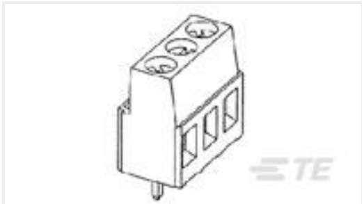
TE 产品编号282843-2 TERMI-BLOK PCB MOUNT 90 2P.1
