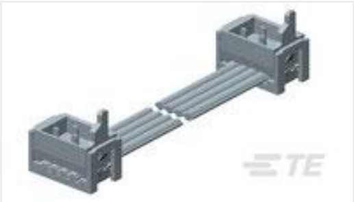
TE 产品编号2205064-1 CA MICRO-MATCH MOW-MOW 12POS
