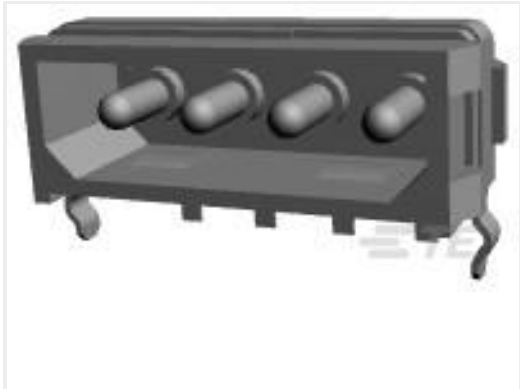
TE 产品编号174552-1 4P C-MNL PIN HDR R/A
