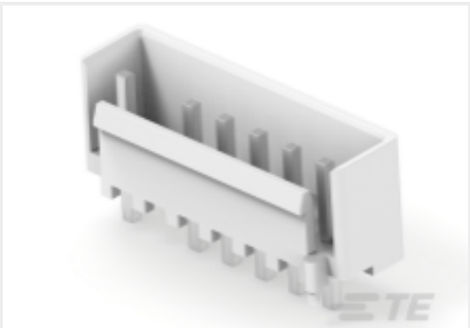
TE 产品编号1-1877285-7 07P EP SHRD HDR ASMY, WHITE,NO PIN 6
