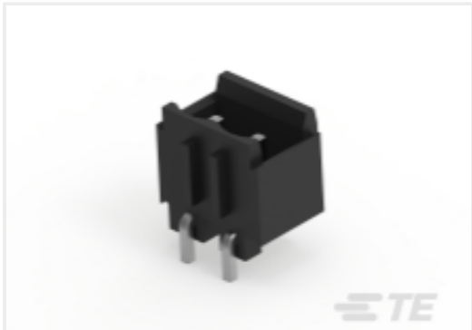
TE 产品编号2305908-2 SMT TB R/A HEADER, 5.0MM, 2 POS
