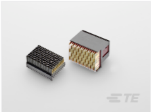
TE 产品编号 2313237-2 RAPLUG ASSY, MGRT3, POWER, DP, SE, CENTER
