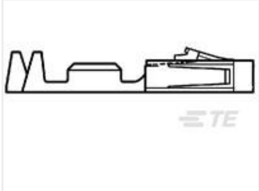
TE 产品编号1-104479-1 SHORT POINT RECP CONT LP
