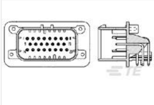
TE 产品编号1-776087-4 23POS,PIN DIA 1.3,HDR ASSY,90DEG, COD 4
