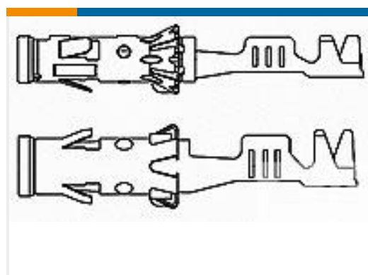
TE 产品编号929989-1 1,5MM SOCK CONTACT
