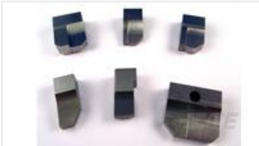
TE 产品编号9-1633131-1 ANVIL, COMBINATION .080
