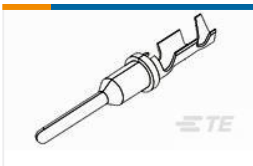
TE 产品编号1924463-3 PIN, SF, SIZE 16, 18-20 AWG, NI/SN
