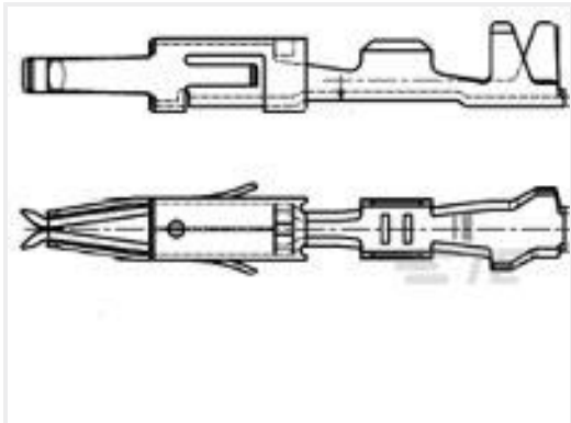
TE 产品编号968052-1 MT3 REC 1.6 Contact SRC Sn
