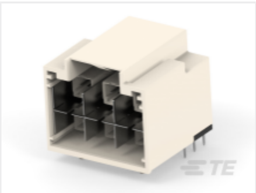
TE 产品编号2339800-2 MATENET 2X3 HEADER, 90DEG, CODE B
