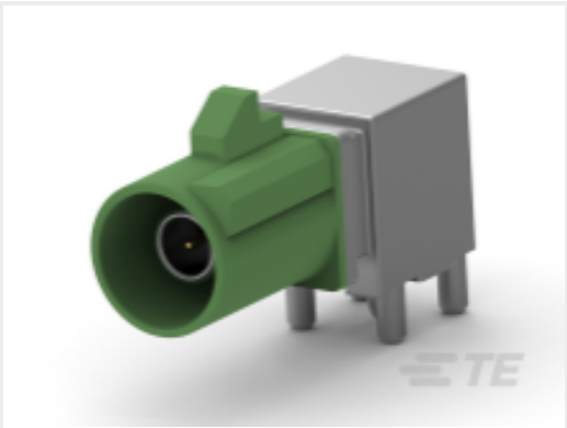
TE 产品编号2291392-5 1POS,FAKRA AUT,HDR OUTER HSG, 90DEG,COD E
