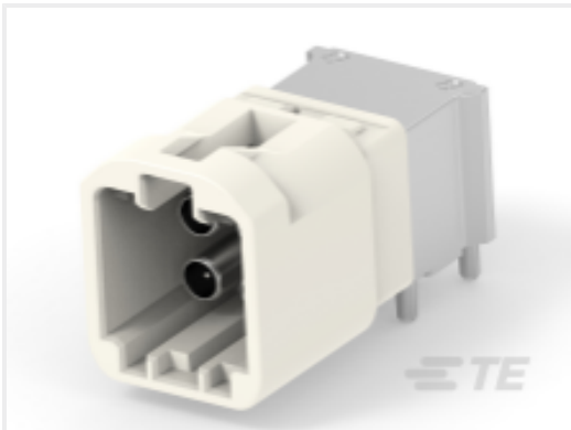
TE 产品编号2405707-2 4P,MATE-AX,HDR ASSY,90DEG,COD B
