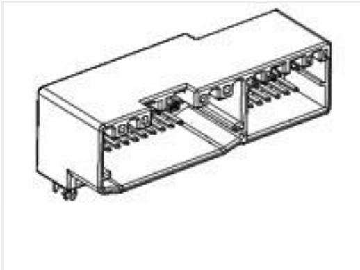
TE 产品编号9-1438743-6 54way Hyb .040/2.8 Tails Down Cap Assy
