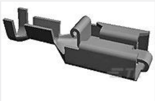
TE 产品编号927854-6 PL 250 REC TERMINAL 17-13 AWG PTPB
