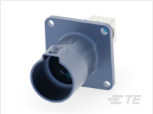
TE 产品编号CAT-AQ4-HHD1400180 PowerTube HVP-HD 1400 180° 接头
