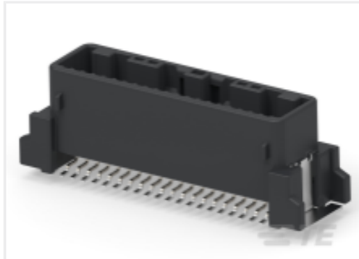
TE 产品编号2321996-1 0.64 SMD 40POSITION CAP ASSEMBLY V-TYPE
