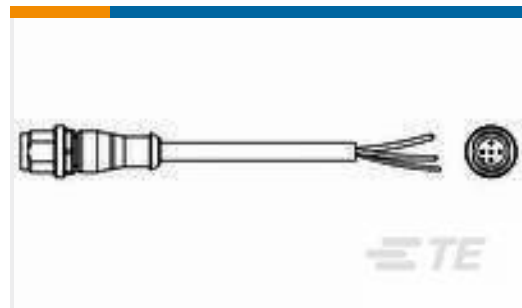
TE 产品编号1-2273028-3 M12 x 1.0 straight plug pigtail A
