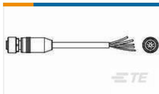
TE 产品编号2273041-3 M12 x 1.0 straight socket pigt A
