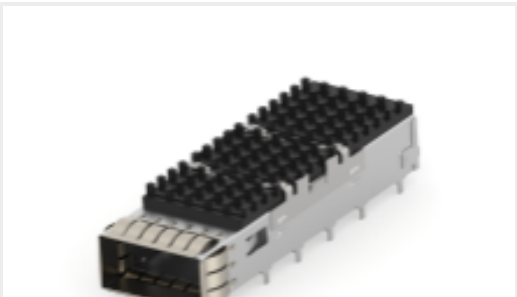
TE 产品编号1-2170704-1 CAGE ASSY, QSFP28 1X1, SPRING, HS
