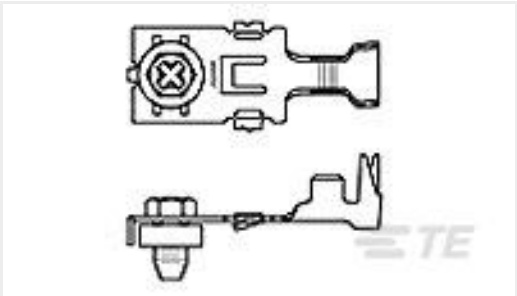
TE 产品编号521844-1 POWER BLOCK ASSEMBLY 16-12 AWG BR
