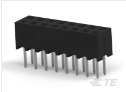
TE 产品编号1-2314812-6 16P,2MM,B-B,REC,DRV,2.0,0.1AU,TB, W/CAP
