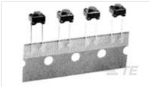
TE 产品编号4-1437565-0 FSM4JRT=FSM 2 LEAD ON RADIAL T
