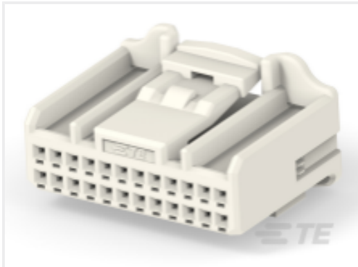
TE 产品编号2321519-1 24POS,TH 025,REC HSG ASSY,UNSLD
