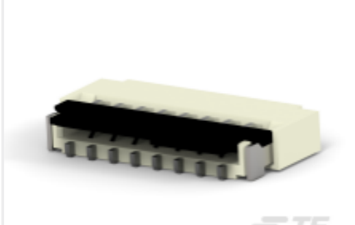
TE 产品编号4-2328724-5 45PIN 0.3MMMP FPC CONNECTOR, FRONT FLIP
