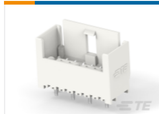
TE 产品编号1-2232960-7 7P POTTED RAST 2.5 HEADER
