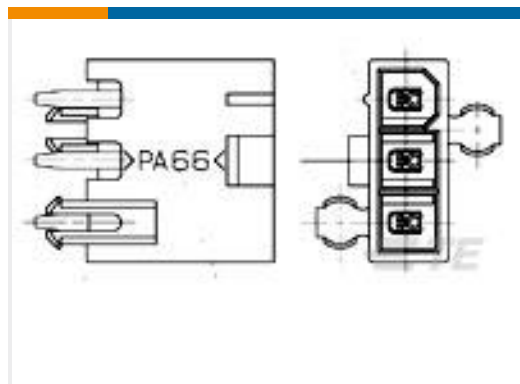
TE 产品编号2029181-5 5P VAL-U-LOK VRTHDR W/PGS GW
