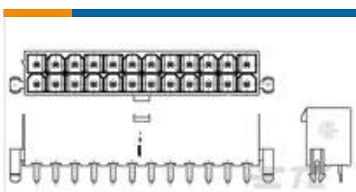
TE 产品编号8-215079-6 Female-on-Board Connector, Top Entry
