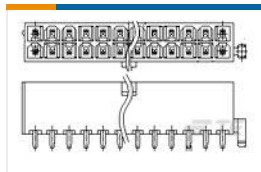
TE 产品编号3-1775099-5 ATX PWR CONN 1 BDLK 14 POS
