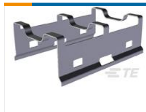
TE 产品编号1489948-2 XFP HEAT SINK CLIP, PLATED
