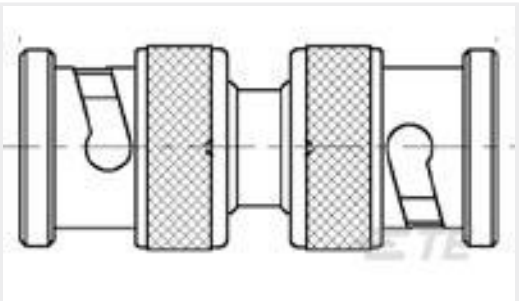
TE 产品编号1-1478043-0 BNC M TO BNC M ADAPTOR,STR,75 OHM,2G
