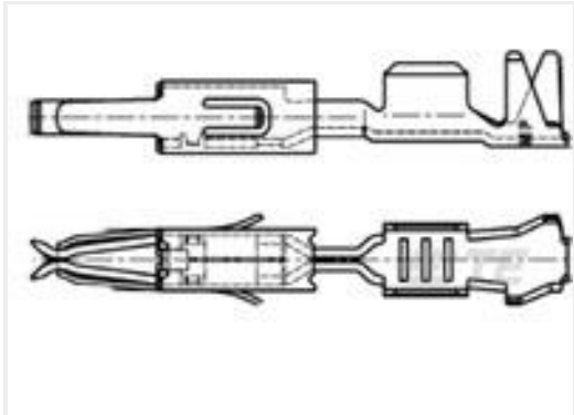
TE 产品编号964261-2 MT2 A REC 1.6 Contact SRC Sn
