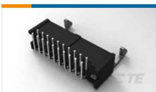
TE 产品编号2-1761607-6 IDC LOW PRO HDR 16P RA LG LAT
