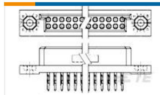
TE 产品编号533289-5 BOX II 2 ROW RECP ASSY 60 POS
