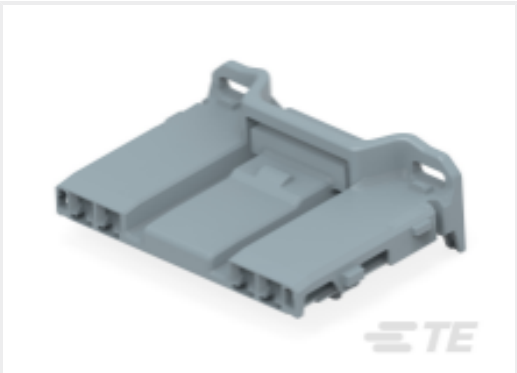
TE 产品编号1-1903607-5 1.5 SERIES CONNECTOR 4POS LOCK HOUSING
