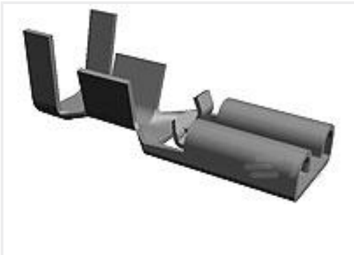
TE 产品编号1217096-2 PL 187 RECEPTACLE 18-14 AWG TPBR
