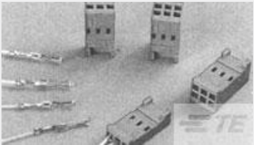
TE 产品编号281839-5 HOUSING HE13 HE14 COSI 2X5 P
