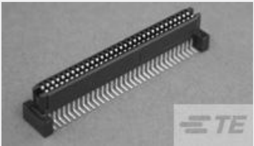
TE 产品编号5120603-2 1FHR,84,30A/S,S,N,S11,12
