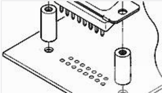
TE 产品编号5205933-4 STANDOFF BUSHING, BULK PACKED
