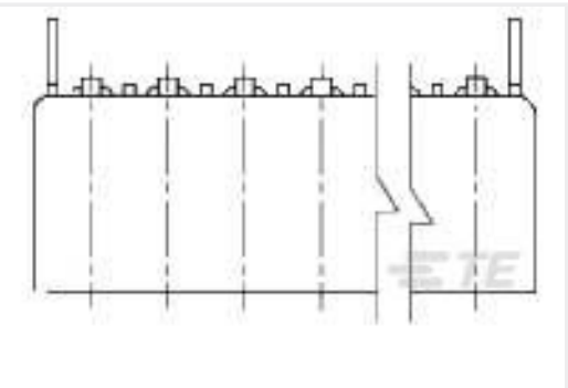
TE 产品编号5-487508-7 TRIOMATE ASY H 8P L=3.175,LDFR
