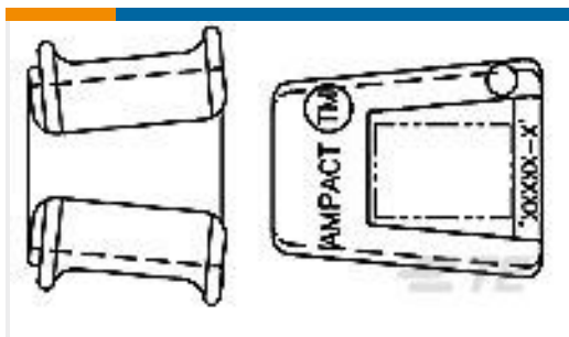
TE 产品编号602006 AMPACT Tap 336.4-266.8
