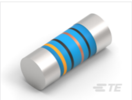
TE 产品编号2176315-7 MELF SMA_A 330R 0.1% 15PPM 0204 0.4W
