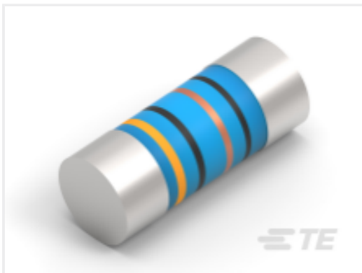
TE 产品编号4-2176315-7 MELF SMA_A 560R 1% 50PPM 0204 0.4W
