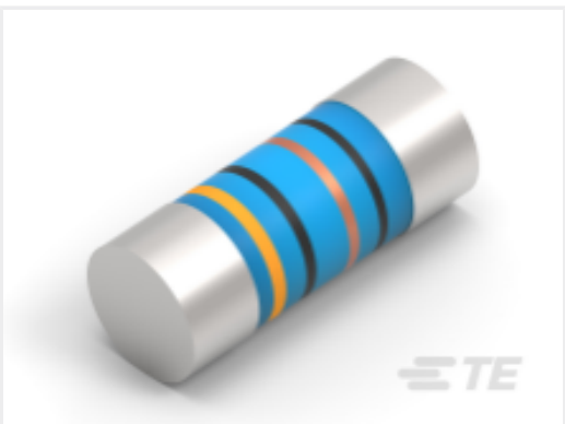
TE 产品编号5-2176315-0 MELF SMA_A 1K0 1% 50PPM 0204 0.4W
