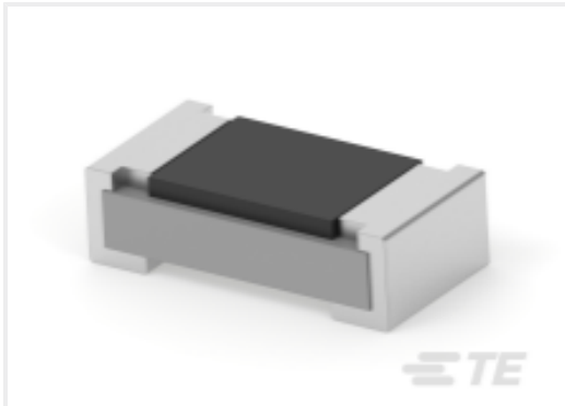
TE 产品编号2176237-8 CPF A 0603 33R 0.1% 25PPM 5K RL
