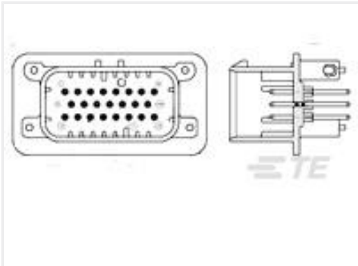
TE 产品编号776228-4 23POS,PIN DIA 1.3,HDR ASSY, 180DEG,COD 4
