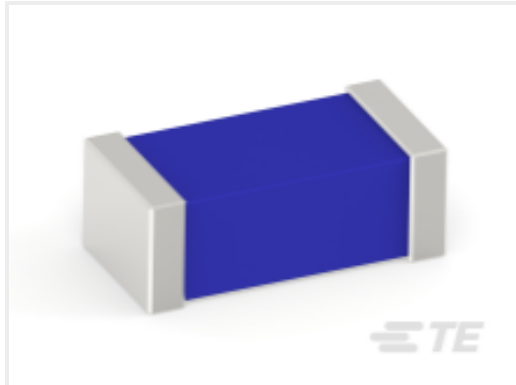
TE 产品编号2108838-1 Chip ant., SMD, BT/Wi-Fi 2.4GHz
