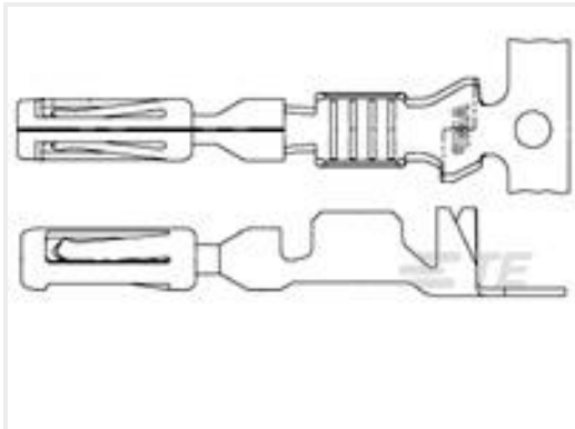
TE 产品编号770520-1 AMPSEAL,TERMINAL,TIN PLATE,16- 20AWG WIRE
