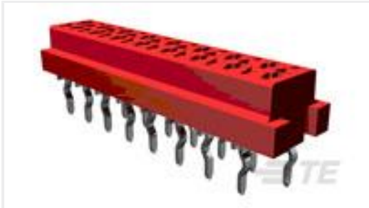
TE 产品编号215079-4 MICRO-MATCH FOB.04P
